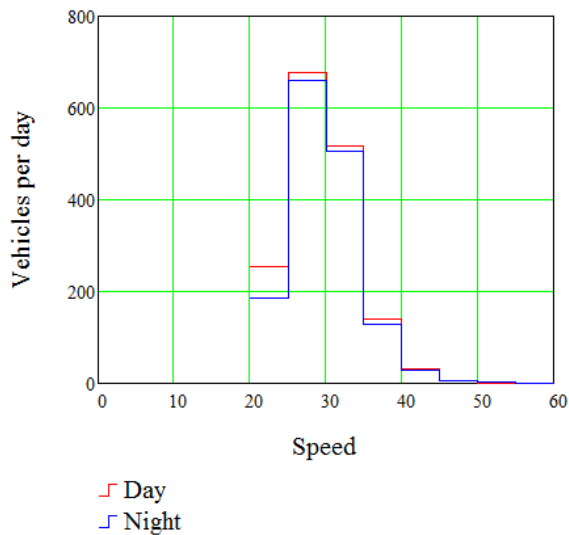
Speed and Number of Vehicles
