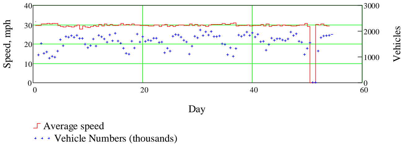
Average speed in each time interval
