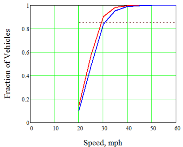
Speed Distribution
