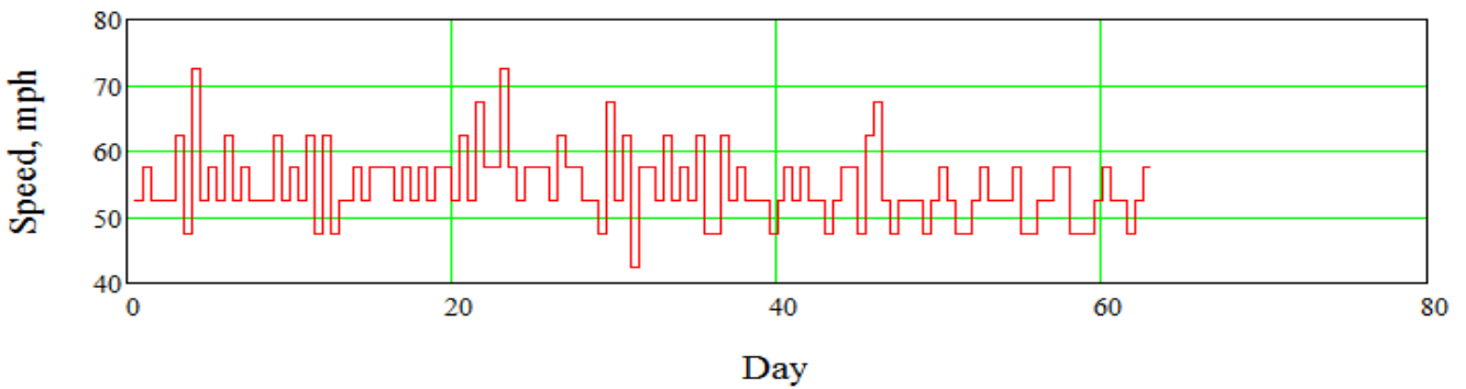
Maximum speed in each time interval
