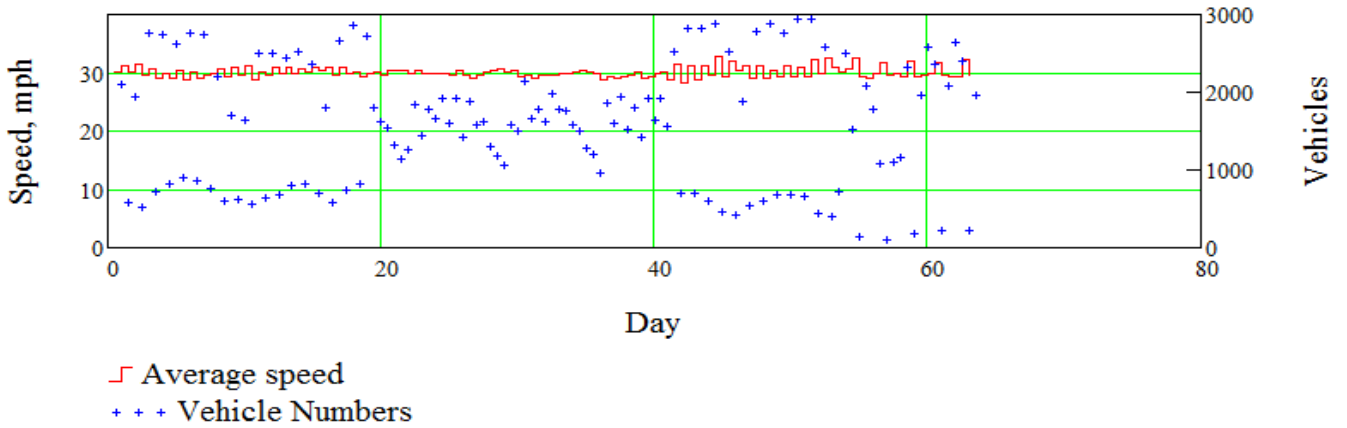
Average speed and numbers of vehicles in each time interval
