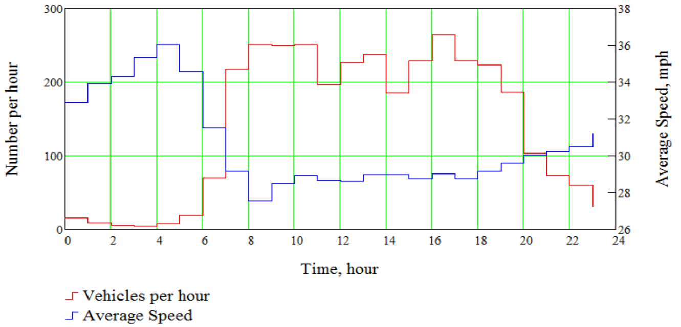
Average Number of Vehicles Per Hour and Speed
